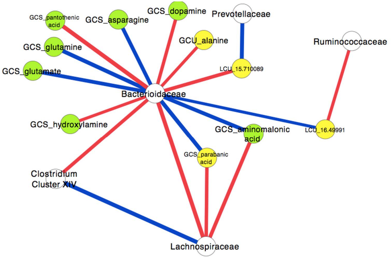
Bacteroidaceae Before
