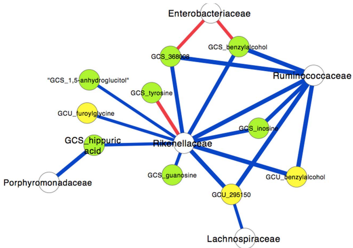
Rikenellaceae After
