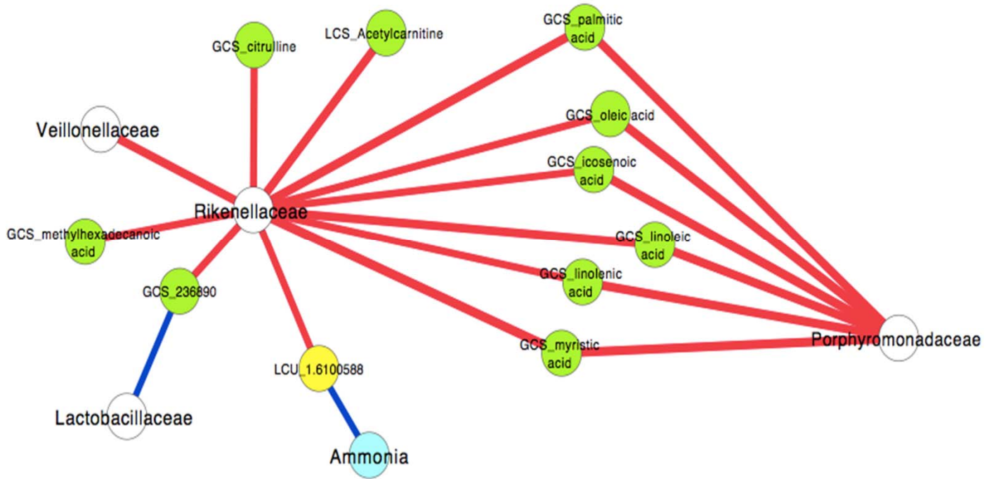
Rikenellaceae Before
