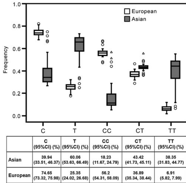
SUPPLEMENTARY FIG. S1. Frequencies of the alleles and genotypes among controls stratified by ethnicities. The “○” and “△” represent outliers.
