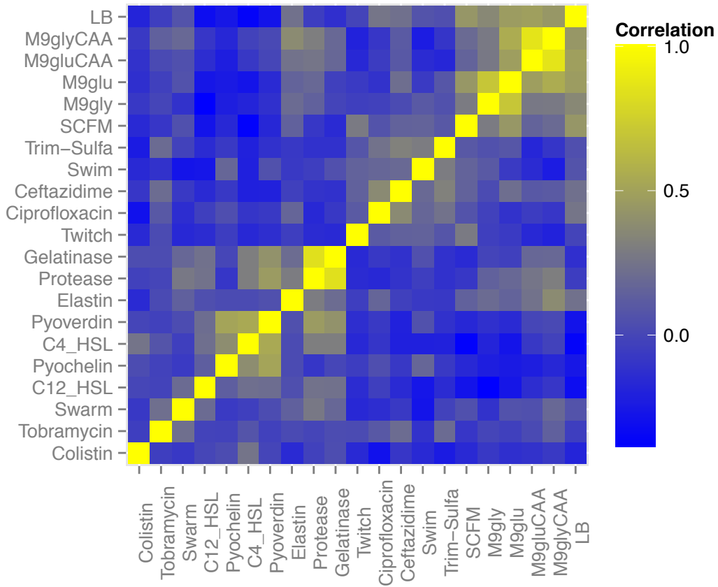
Figure S4. Correlation matrix of the measured phenotypes. The Pearson correlation coefficient was calculated for each phenotype pair where the yellow represents a high correlation (close to 1) and blue represents no correlation (close to 0).
