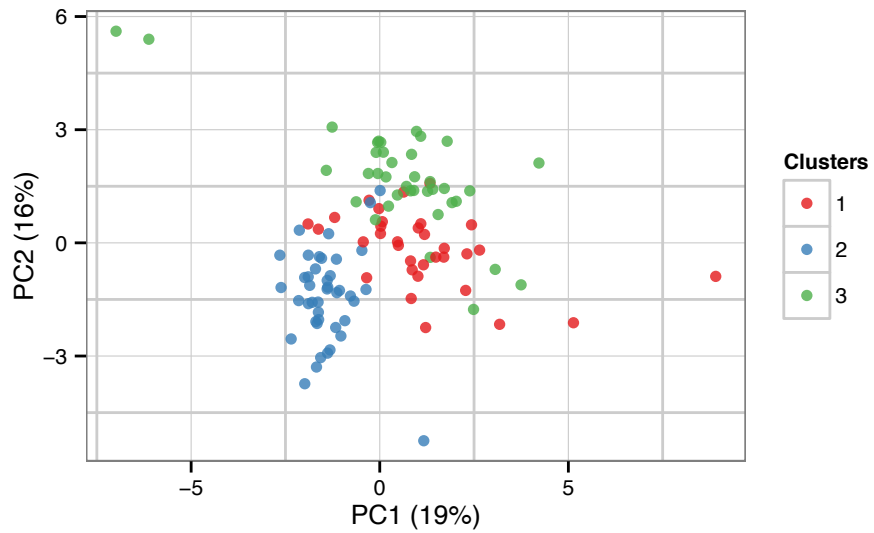
Figure S7. PCA analysis of the measure phenotype profiles. The first two components are shown and the data points are coloured according to the cluster pattern observed in the hierarchical cluster analysis. The amount of variation (in percent) explained by each principle component is shown on the axis.
