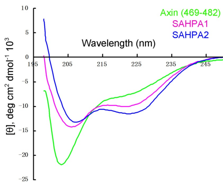
Supplementary information, Figure S1 Circular dichroism spectroscopy of SAHPAs illustrates the incremental effects of synthetic modification.
