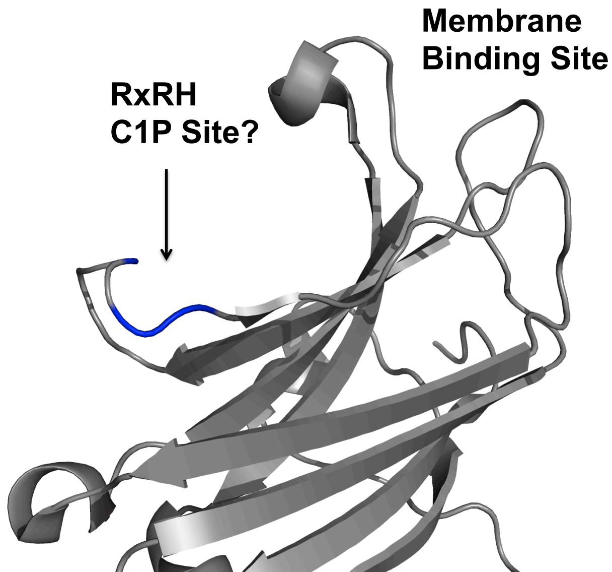
Fig. S2. Structure of the RGP3 C2 domain. The C2 domain of RGP3 (PDB ID: 3FBK) harbors a putative membrane binding site similar to other C2 domains as well as a RxRH motif in a similar position to that of the C2 domain of cPLA 2 \alpha .
