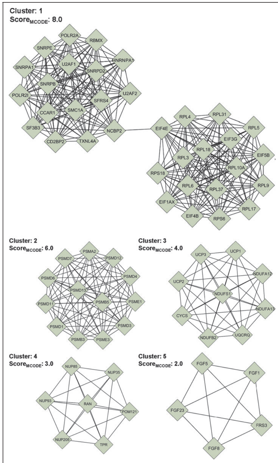
Supplementary Fig. S3. Top 11 highly interconnected gene clusters from the 1,252 nominated essential gene candidates. The cluster number and MCODE score is included. ( continued )
