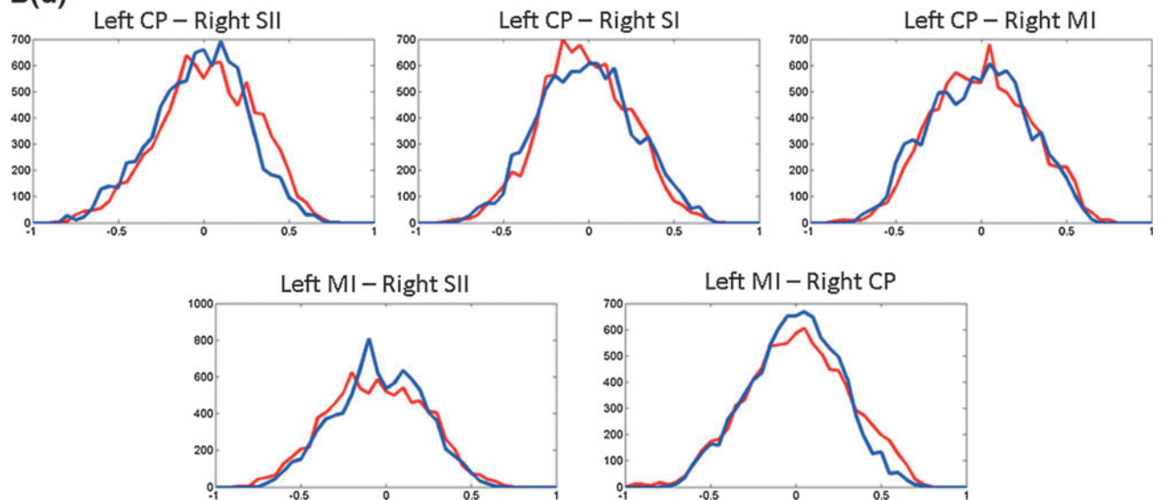
SUPPLEMENTARY FIG. S1. (Continued).
