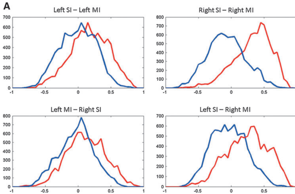
SUPPLEMENTARY FIG. S1. Histograms of correlation coefficients after sliding window correlation with a window length of 50 images (all rats, all scans). Real data are shown in red, and results for randomly matched time courses are shown in blue. (A) Histograms for SI-MI connections, which are shifted to positive values and sometimes skewed as compared with the randomized data. (B) Histograms for the remaining pairs of areas, which are similar to those for random data. Histograms for homologous areas in left and right hemispheres were shown in Figure 4.
