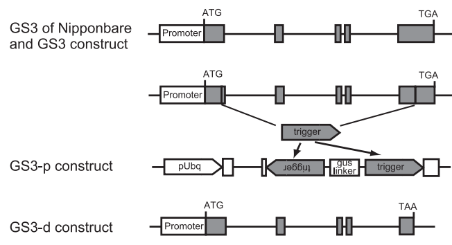
Supplemental Fig. 1. The construct designs used for transformation (the GS3 construct, GS3-p construct and GS3-d construct).
