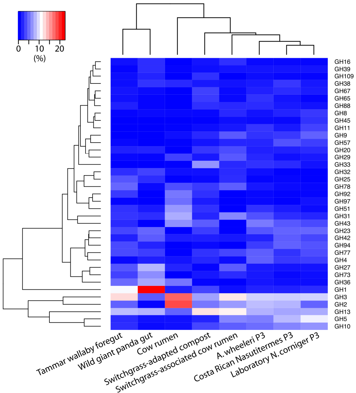
Figure S6. A cluster heatmap showing the clustering patterns of lignocellulose-degrading communities based on GH composition (the relative abundance of individual GHs in total GHs, based on gene counts). Only the GHs with the relative abundance \geq 2\% in any one of these microbiomes were shown in this heatmap.
