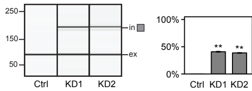
SUGP2
