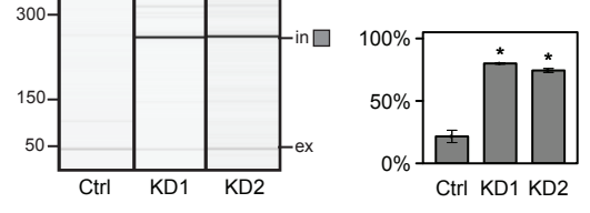
ZFX
