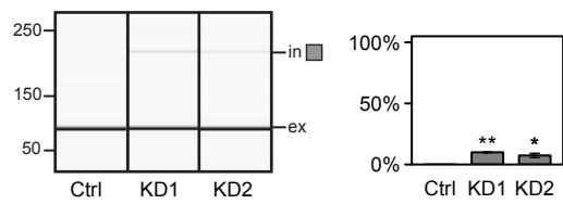
SSR1
