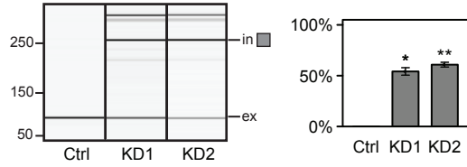
SPG7
