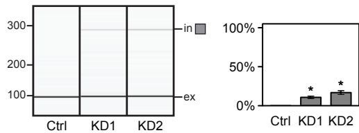
TCFL5
