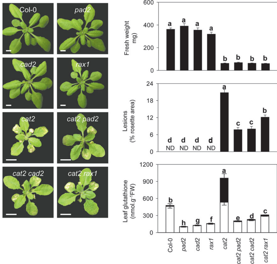
SUPPLEMENTARY FIG. S1. Confirmation of effects of genetic deficiency in glutathione (GSH) on H 2 O 2 -triggered lesion formation using allelic mutants.
