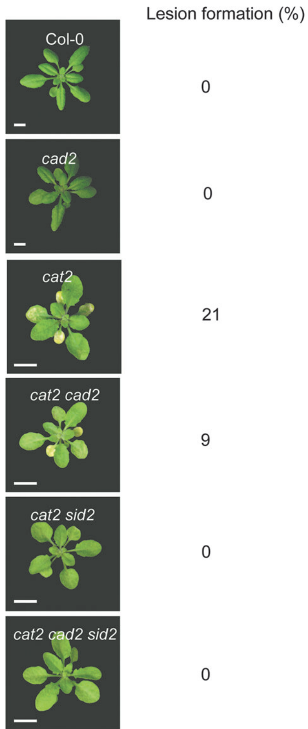
SUPPLEMENTARY FIG. S2. The cat2 cad2 sid2 triple mutant shows that residual H 2 O 2 -induced lesions in cat2 cad2 are dependent on the isochorismate synthase (ICS1) pathway.
