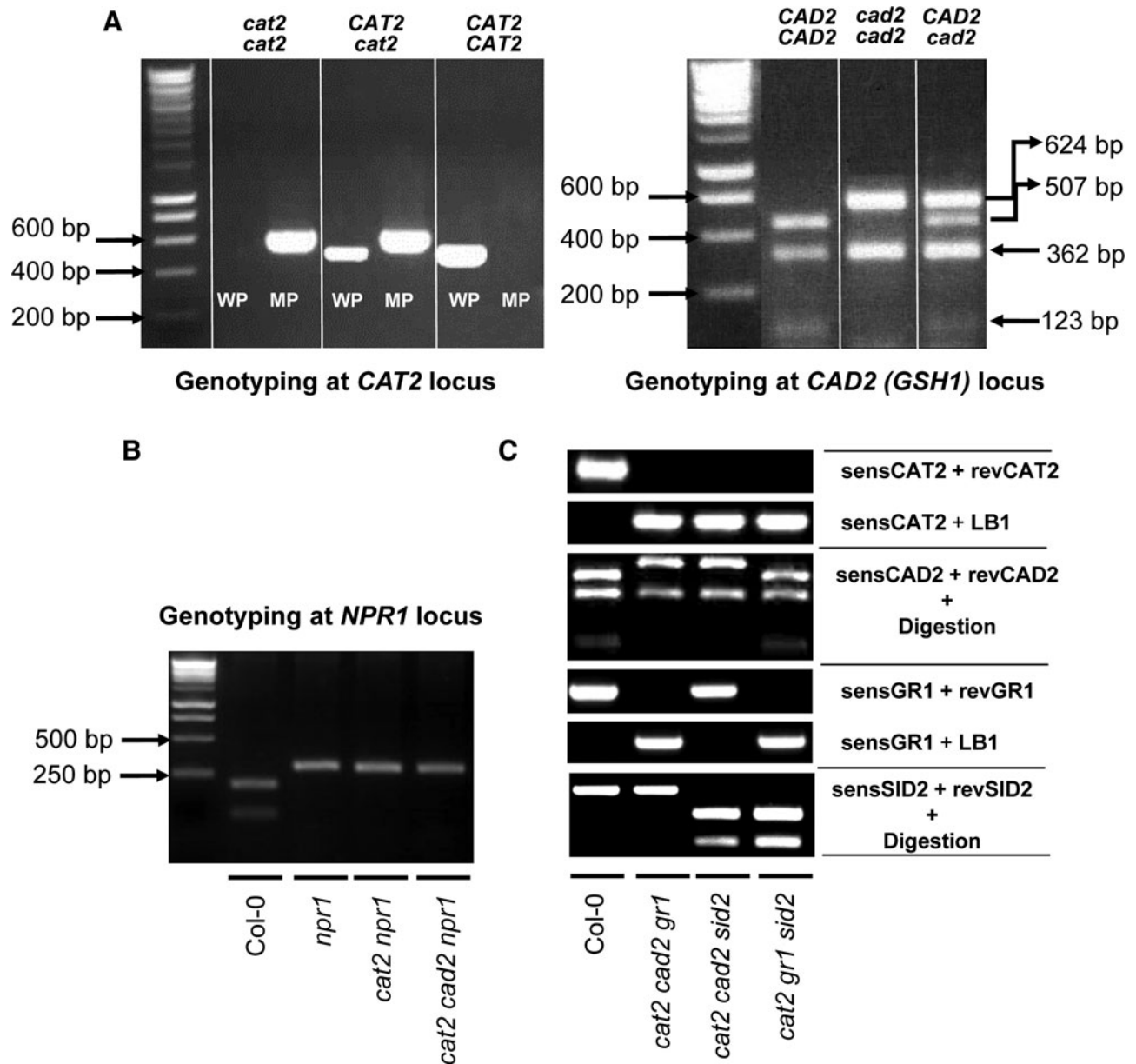
SUPPLEMENTARY FIG. S6. Genotyping of double and triple mutants. (A) Genotyping of cat2 cad2 mutant. MP, mutant primer pair. WP, wild-type primer pair. (B) Genotyping at the NPR1 locus to obtain cat2 npr1 and cat2 cad2 npr1 mutants. (C) Genotyping of other triple mutants by crossing cat2 cad2 with cat2 sid2 (Chaouch et al. , 2010) and cat2 gr1 (Mhamdi et al. , 2010a).
