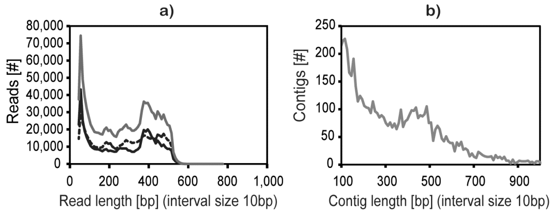
Figure S5. (a) Distribution of the length of the original 454-reads. (b) Sequence length distribution of contigs assembled with Newbler 2.5, removing contigs with sequence length <100 bp; (— = ozone.454-reads, - - = control.454-reads, ··· = ensemble)
