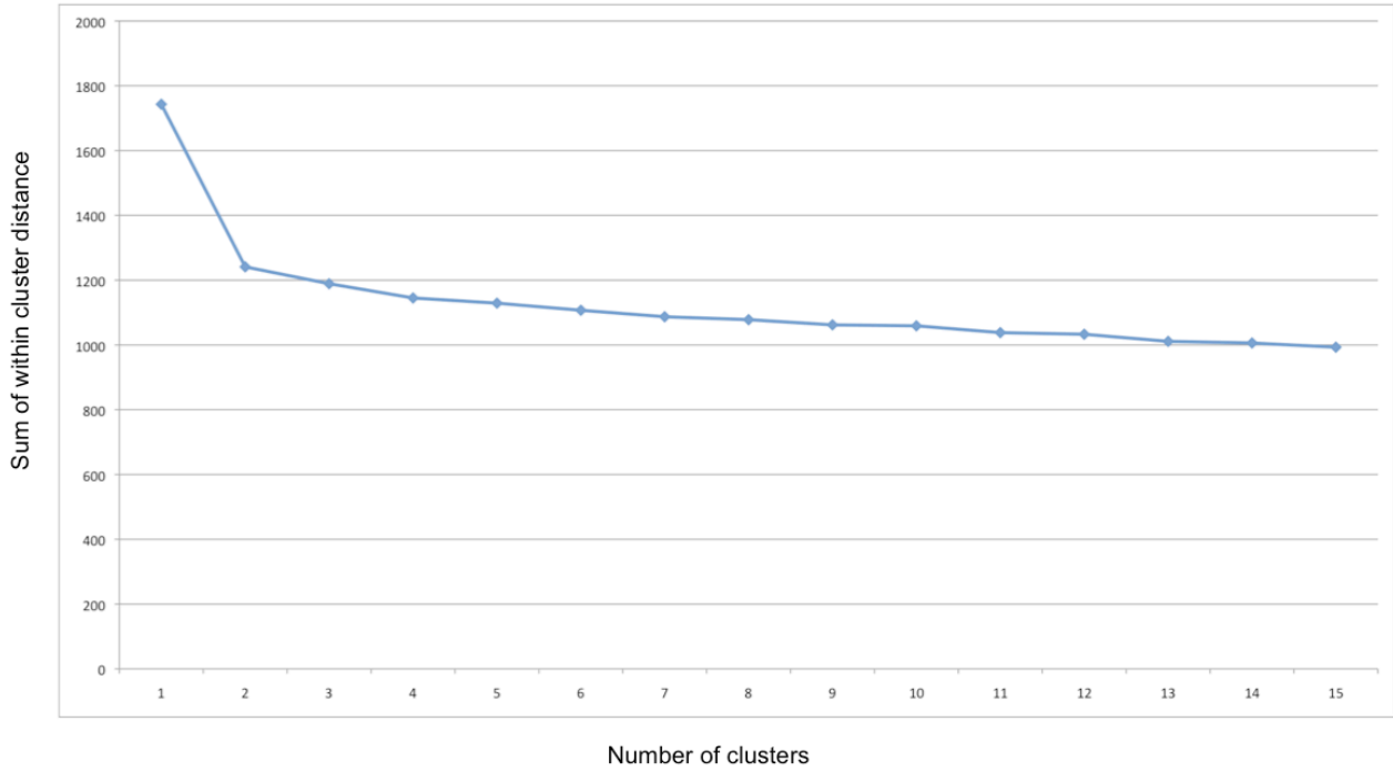
Fig. 1 - Number of clusters selection.
