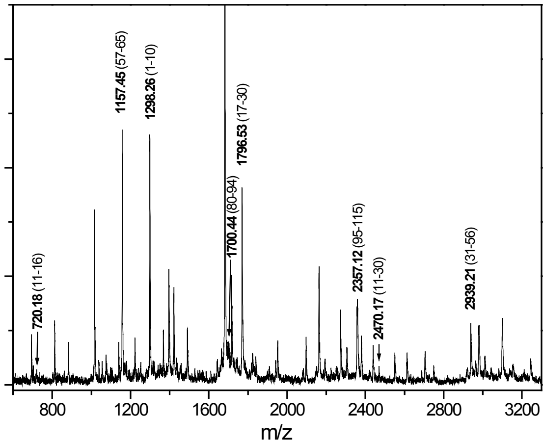
Figure S1. MALDI-TOF analysis of tryptic peptides derived from NNOPLA 2 . The molecular masses and sequence fragments are marked in the figure.
