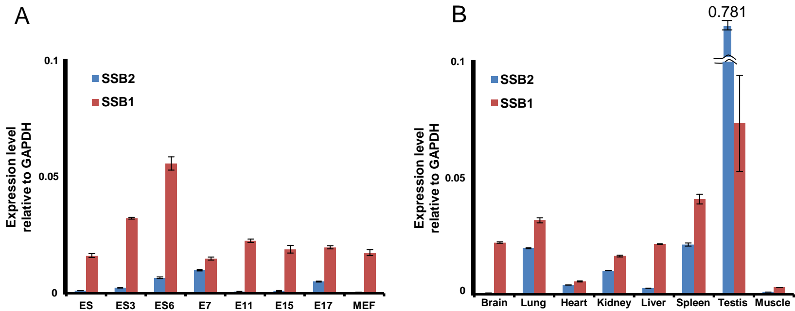
Figure S6 Expression profiles of mSSB1 and mSSB2 transcripts during mouse development A and in different tissues from adult mice B . Total RNAs isolated from ES cells differentiated by addition of retinoic acid for days 0, 3, 6 days. In addition, RNA from day E7 to E17 embryos, E12.5 MEF and indicated adult tissues (Clonetechn RNA library) were subjected to quantitative RT-PCR. Experiments were performed in triplicate. Error bars: s.e.m.
