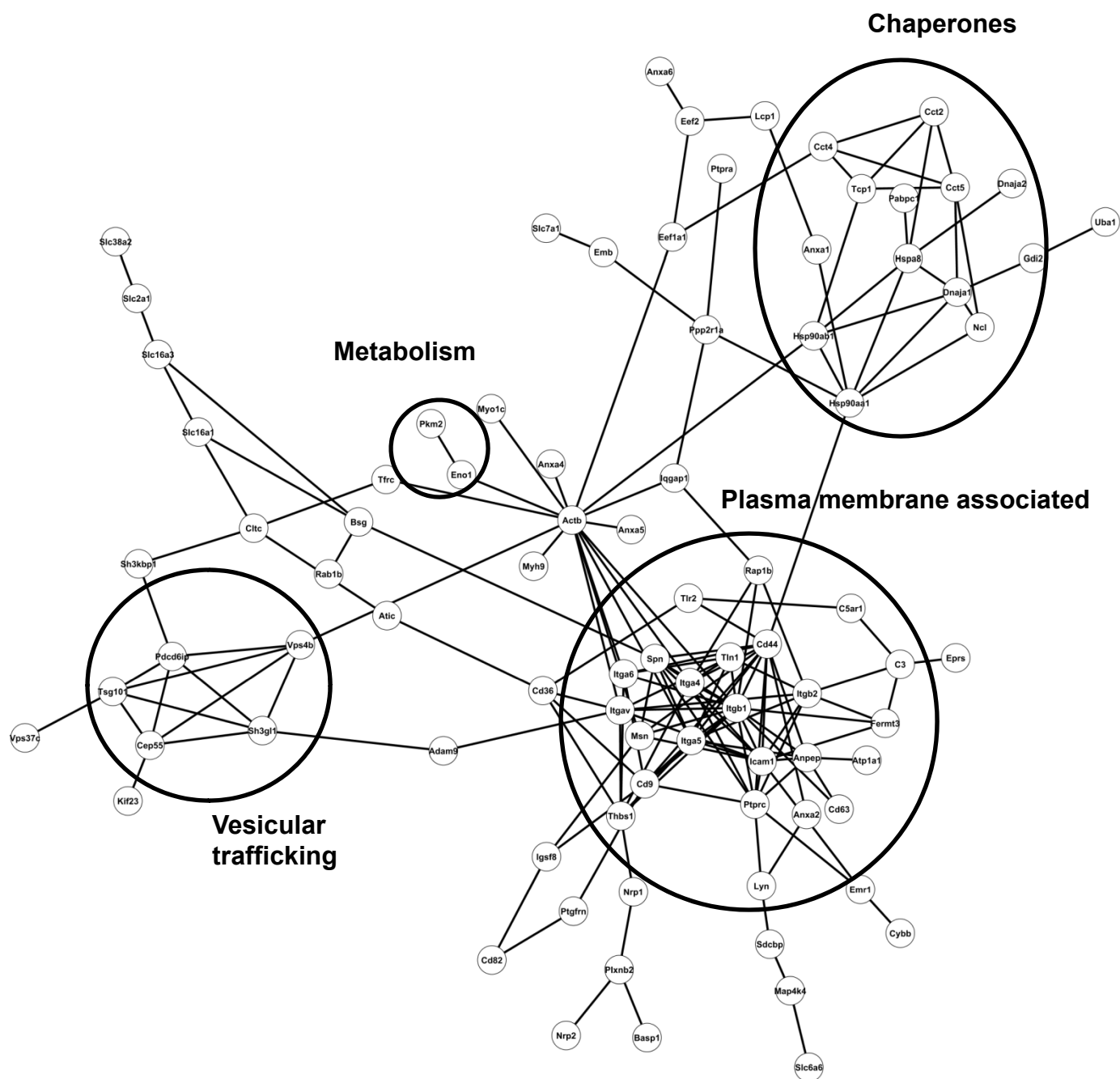
Supplemental File S5. NILX PPI network and the interaction groups of proteins with related functions.
