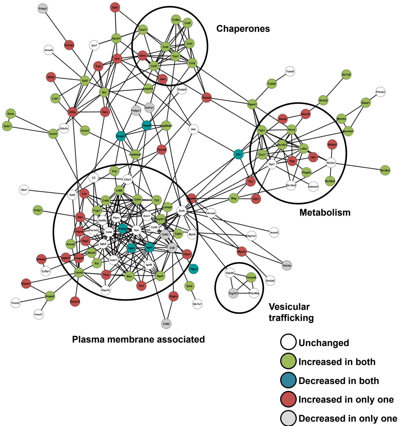
Supplemental File S5. Continued. LEISHX PPI network and the interaction groups of proteins with related functions.
