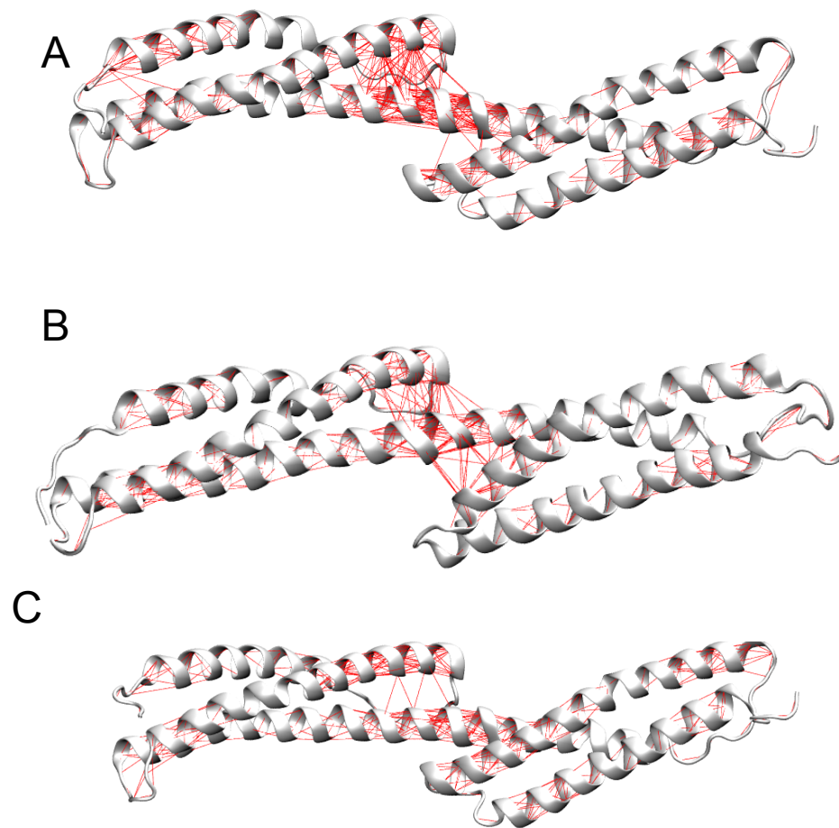
Figure S5: Correlated motions of \text{Ca} residues belonging to 1S35 (A) ^{\text{NES1}} SR70-71 and ^{\text{NES2}} SR52-53 (C). Motions with >80\% correlation are indicated by lines connecting the involved residues.
