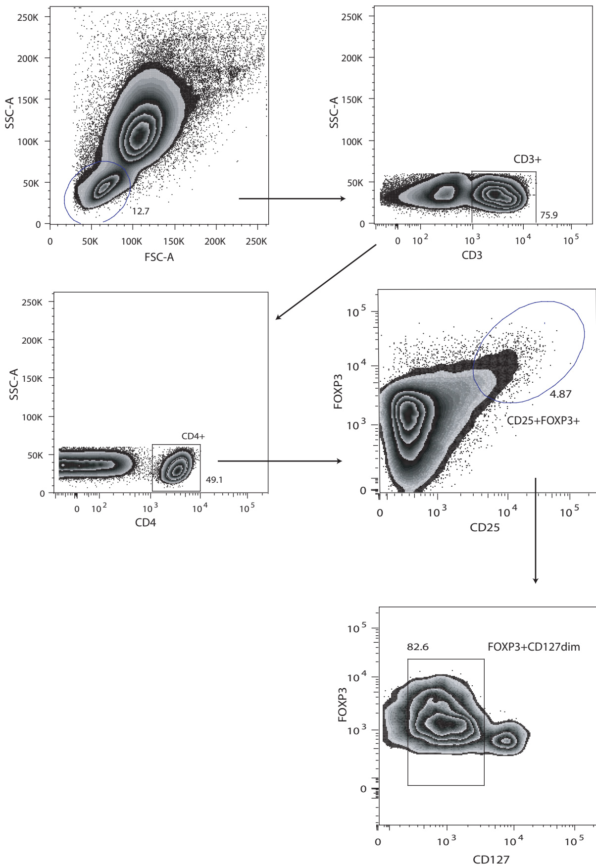
Figure S3. Gating strategy for estimating frequencies of CD4+ nTregs. A representative flow cytometry plot showing the gating strategy for estimation of nTregs. nTregs were classified as CD4+CD25+Foxp3+CD127dim.
