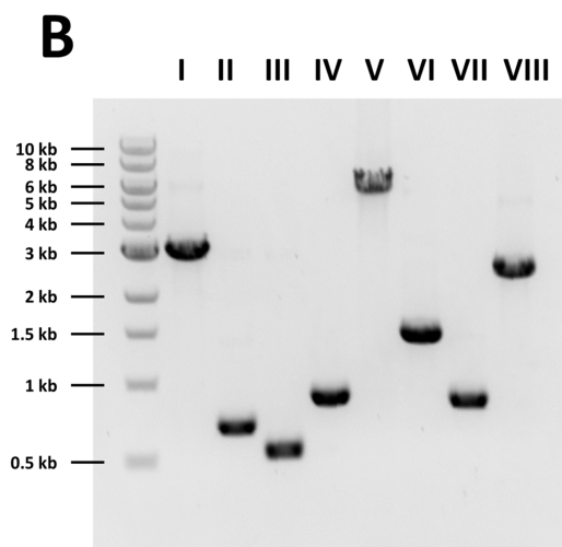
Figure S1. Scheme of Cg_UPC2A and Cg_AUS1 deletion in C. glabrata with PCR verification of deletion cassette integration.
