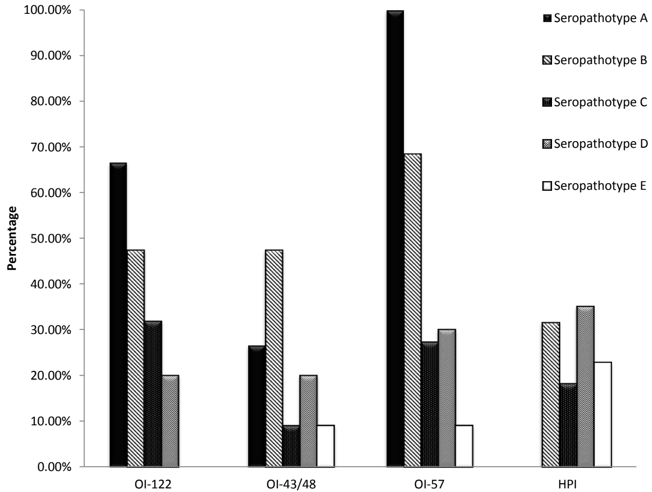
Figure S1. Distribution of OI-122, OI-43/48, OI-57 and high pathogenicity island (HPI) in STEC strains (n=98) of different seropathotypes.
