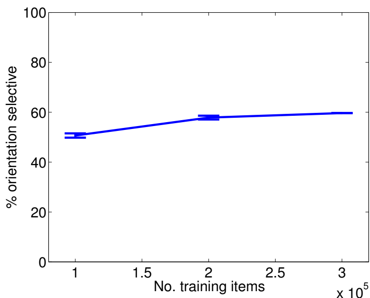
Figure 5. Model is robust to training set size (kmeans model).
