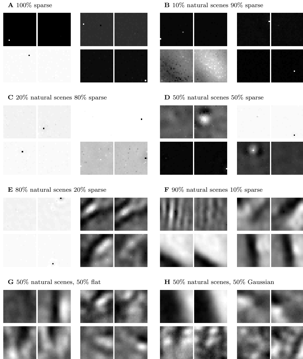
Figure 9. Example receptive fields learned with mixtures of natural scenes and noise (kmeans model).
