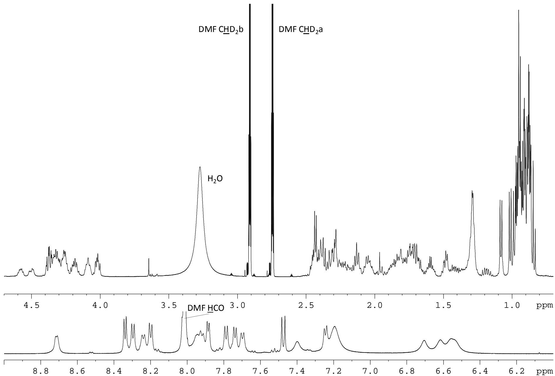
Figure S8. 1D NMR analysis of xantholysin A. 1D ^1\text{H} spectrum of xantholysin A in \text{DMF-d}_7 solution, 55^\circ\text{C} , 500 MHz.
