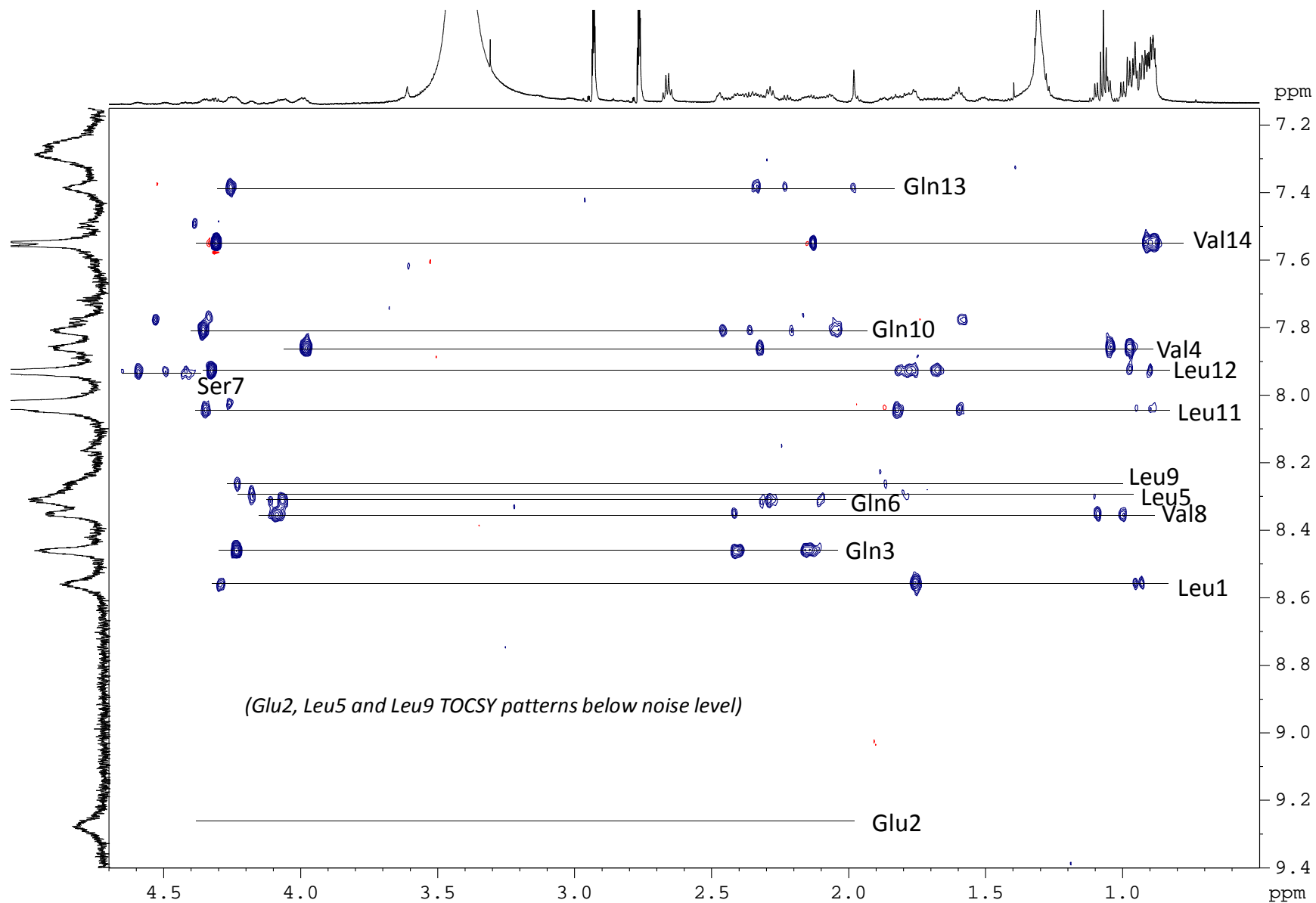
Figure S14. 2D NMR analysis of xantholysin B. 2D ^1\text{H} - ^1\text{H} TOCSY spectrum of xantholysin variant 1, in DMF- d_7 solution, 55°C, 700 MHz, revealing the characteristic amino acid spin system patterns.
