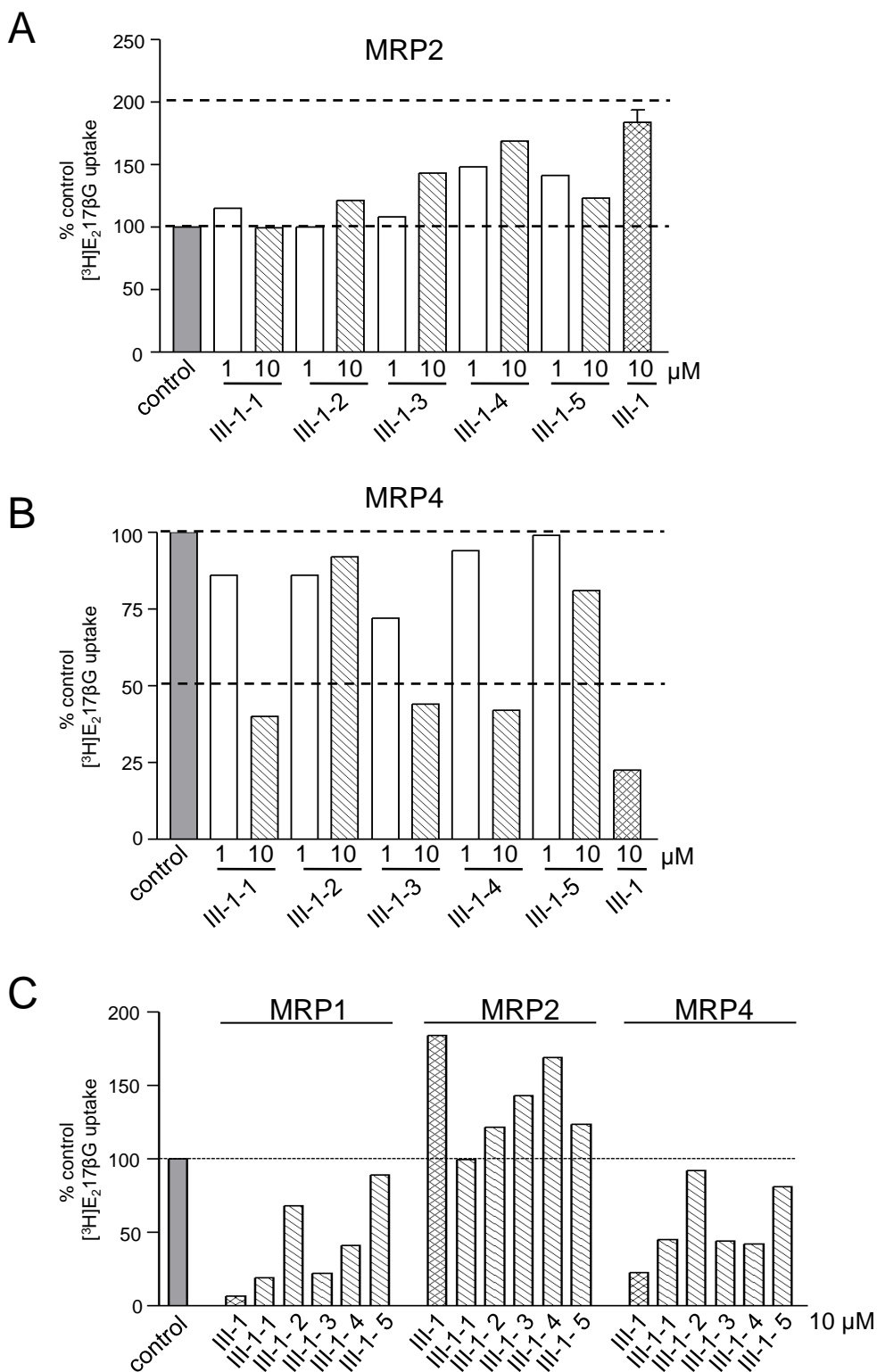
FIG. S3. Effect of CGP III-1 analogs on MRP1, MRP2 and MRP4 transport activities.
