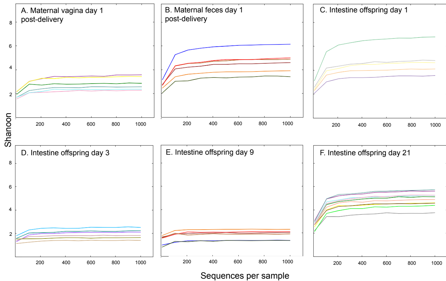
Figure S15. Rarefaction curves of Shannon index from mothers and offspring mice. Panel A, maternal vagina, day 1 post-delivery; Panel B, maternal feces, day 1 post-delivery; Panel C, offspring intestine, day 1 of life; Panel D, offspring intestine, day 3 of life; Panel E, offspring intestine, day 9 of life; Panel F, offspring intestine, day 21 of life.
