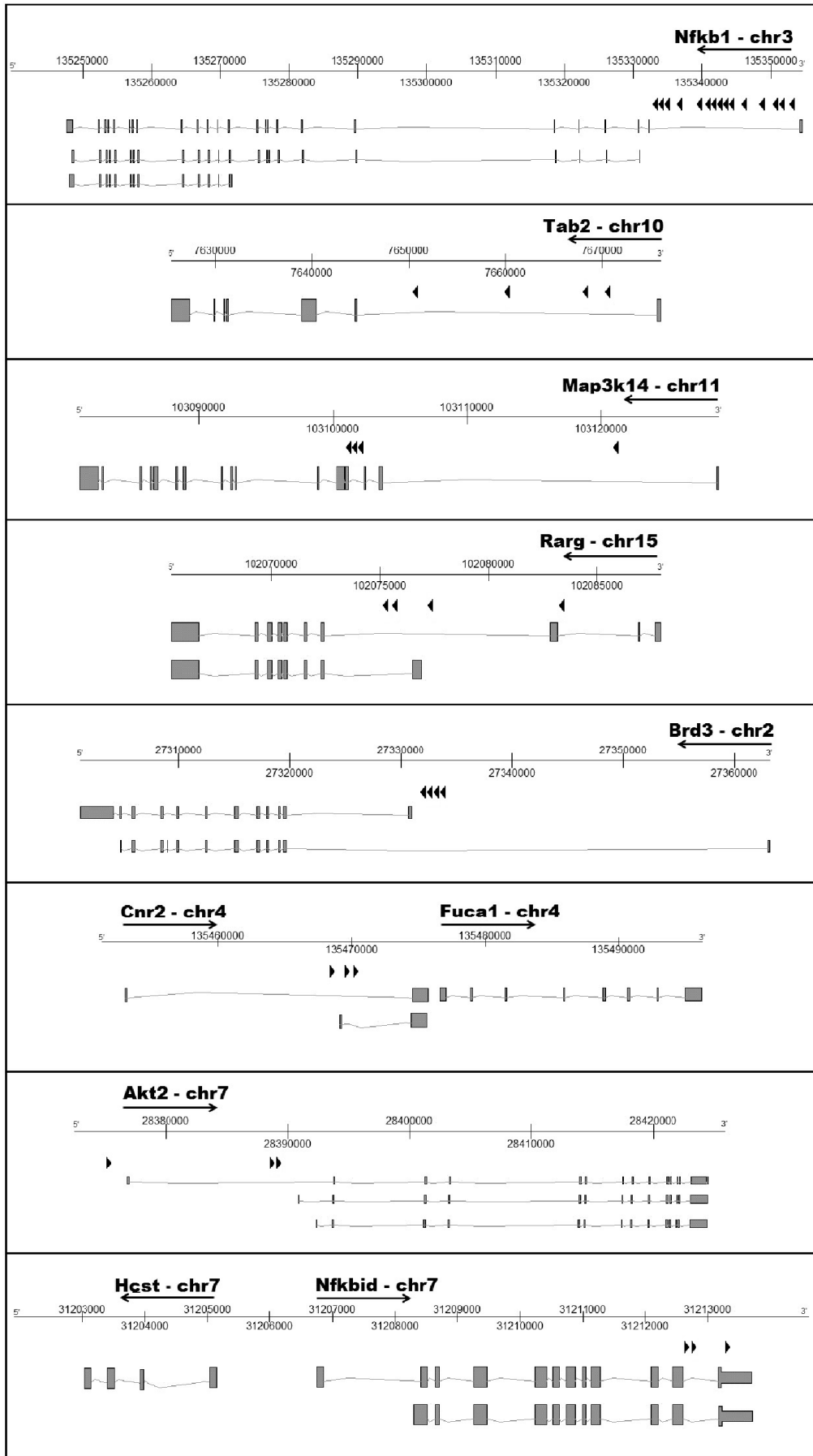
Suppl. Fig. 1. Positions of transposon insertions within affected genes (mouse genome assembly mm9). Locations and directions of transposon insertions are shown as solid arrowheads. Only major transcripts are shown.
