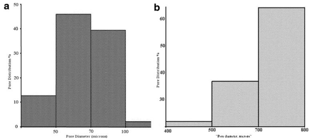
SUPPLEMENTARY FIG. S1. (a) Histogram showing the distribution of pore sizes in the porous scaffold from the liquid extrusion porosimetry experiment using Galwick. (b) Histogram showing the distribution of pore sizes in the porous scaffold from the liquid extrusion porosimetry experiment using Water.
