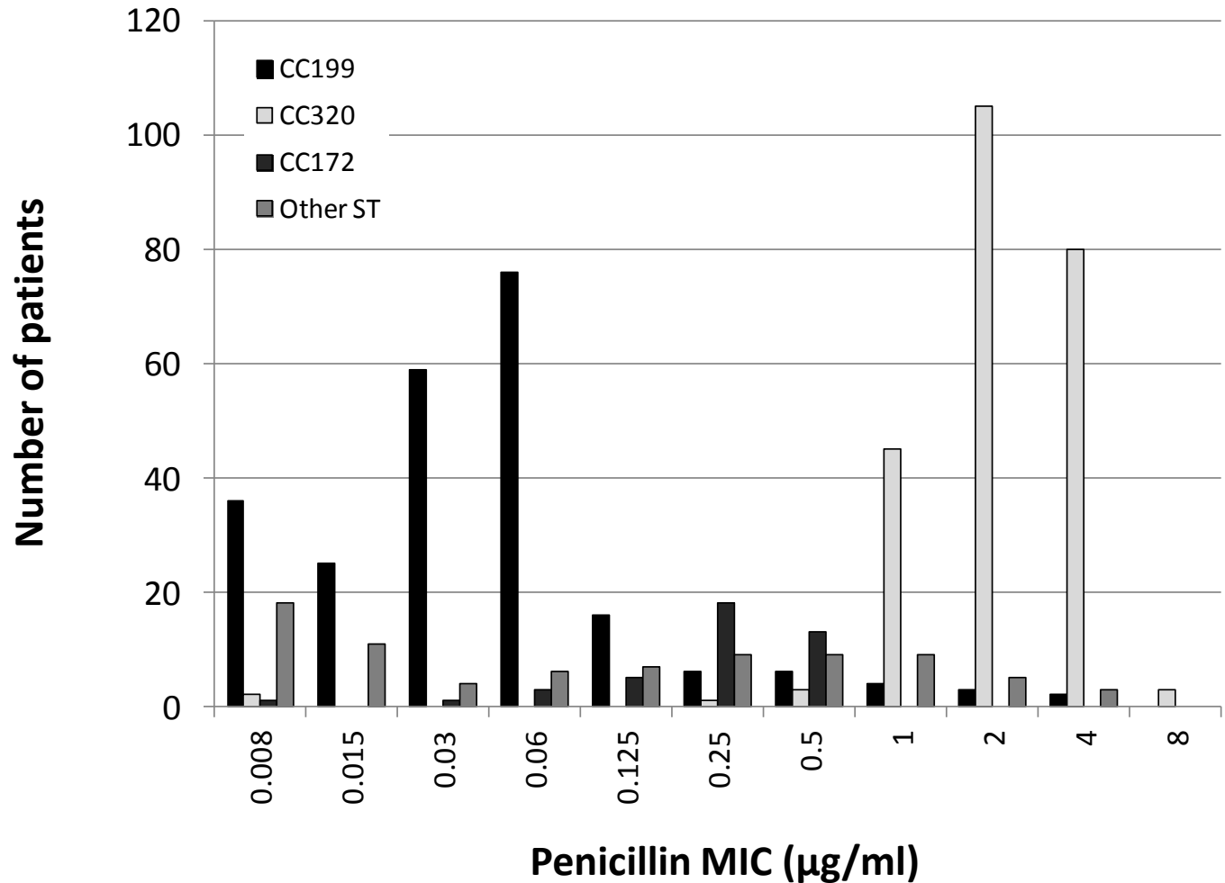
Fig. S1. Penicillin MIC distribution of serotype 19A isolates recovered from 8 children’s hospitals 1993-2011. The isolates were grouped by the most common clonal clusters CC199, CC320, CC172, and “other ST”.
