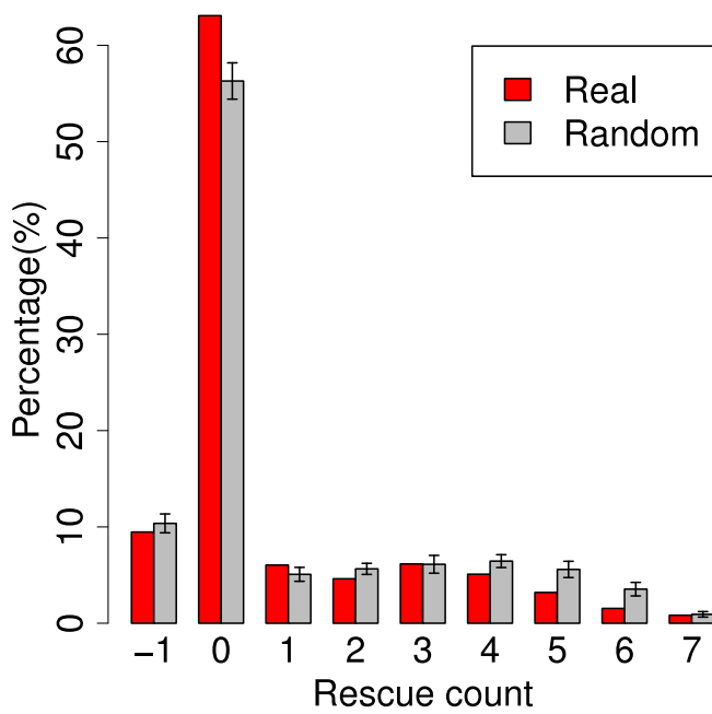
C. Human
