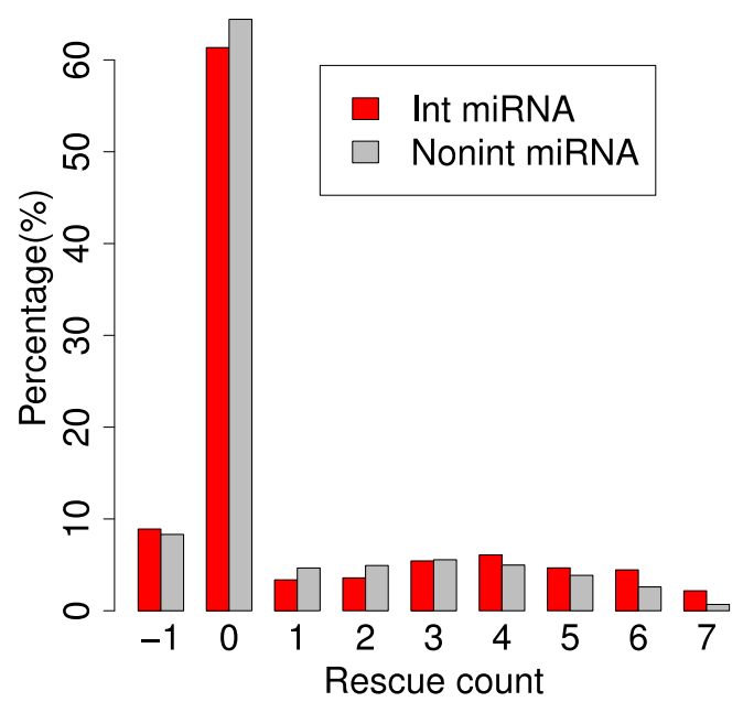
B. Mouse
