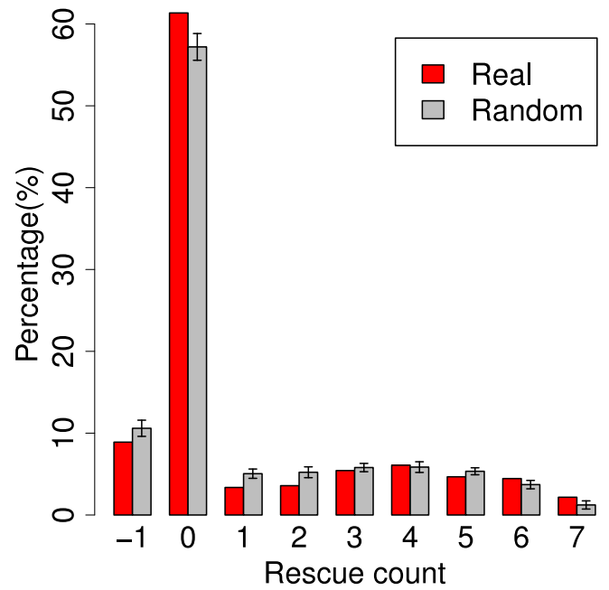
D. Mouse
