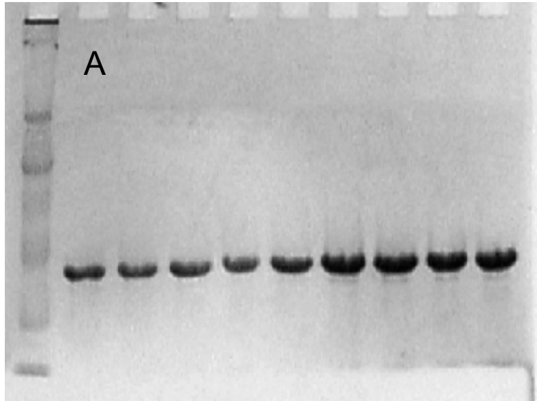
DSS protein
