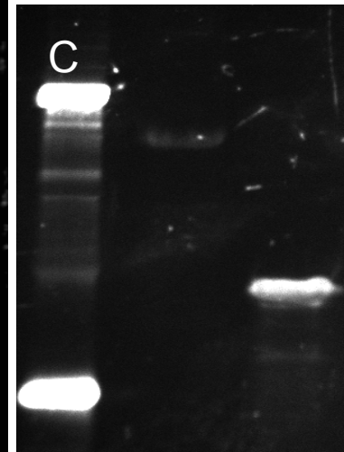
FITC GST-DSS
