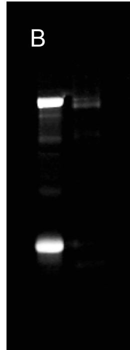
FITC DSS-Runx2
