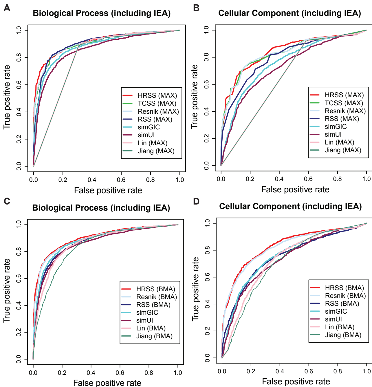
Figure S1. ROC curves comparing different methods based on the human protein-protein interaction datasets (including IEA). The evaluation was carried out for the BP and CC ontologies. The (A and B) maximum (MAX) and (C and D) best-match average (BMA) pairwise rules were used in the ROC analysis.
