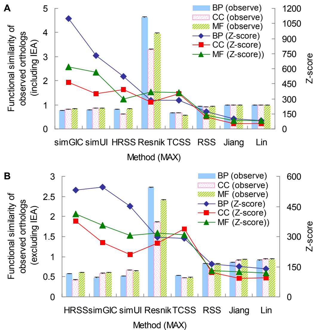
Figure S4. Statistical significance of system for evaluating the functional similarity (MAX) of human-mouse orthologs. The evaluation system was based on BP, CC and MF ontologies (A) including or (B) excluding IEA annotations. The histograms (measured on the left y-axis) indicate the mean and standard error of the functional similarities of observed orthologs, and the lines (measured on the right y-axis) show the Z-score values calculated from the ASVs of observed orthologous pairs and randomized pairs (see Materials and Methods). Error bars indicate one standard error.
