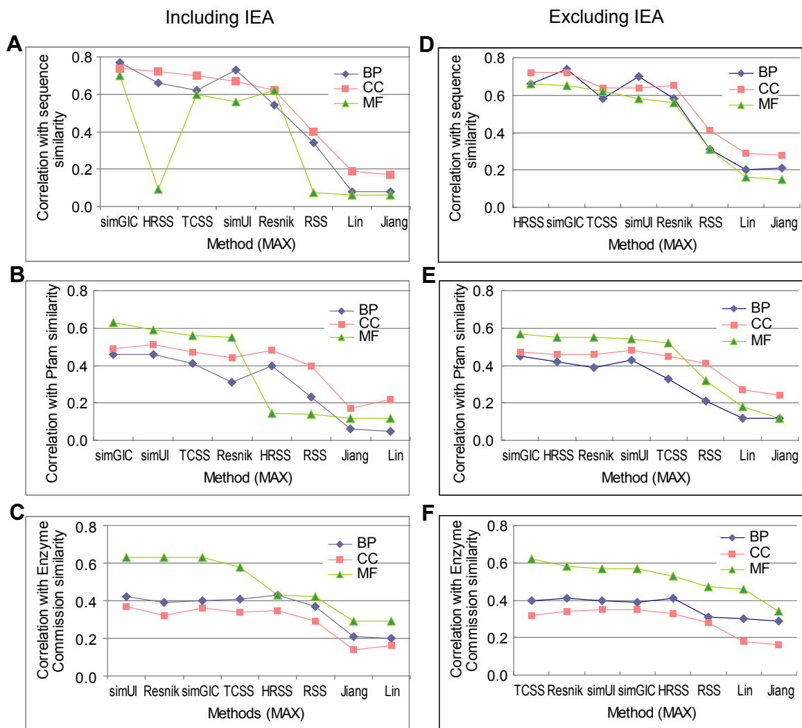
Figure S6. Correlation between semantic similarity (MAX) and the CESSM dataset (including and excluding IEA). CESSM holds the data of (A and D) sequence, (B and E) Pfam and (C and F) ECC similarities.
