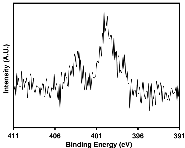
Figure S1. XPS data of SAM-modified silicon substrates confirms the presence of terminal azides. The photoelectron spectra of the nitrogen 1s binding energies shows the two peaks at 400 and 404 eV that are characteristic of azides. 7
