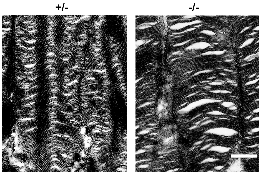
Figure S2 Electron micrographs of outer segments of Dlic1 +/- and Dlic1 -/- photoreceptor cells show well packed disk membranes in both control and mutant OS. [Bar=250 nm]
