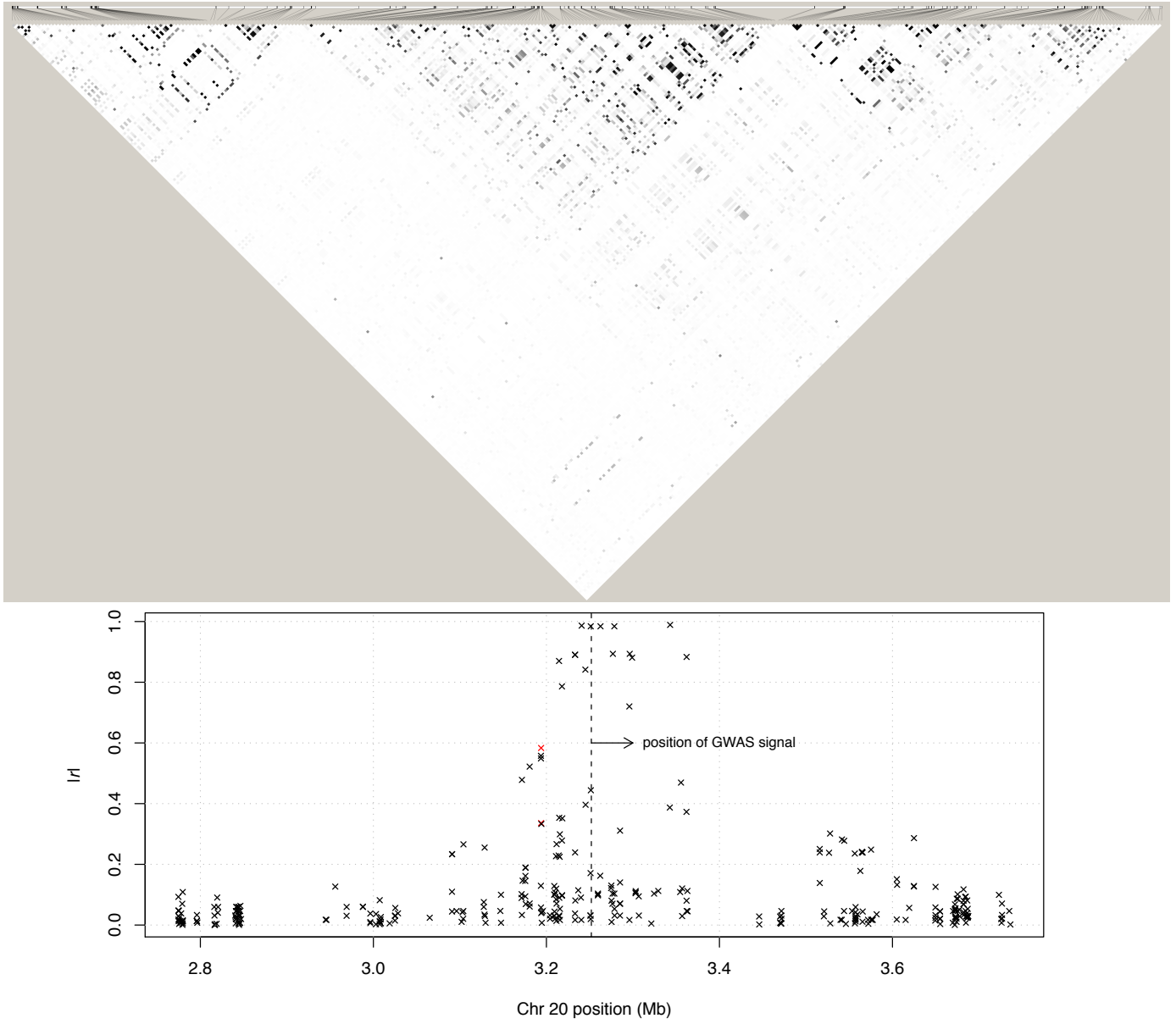
Figure S 2: Same as Figure S1 but for the 338 candidate variants in ITPA region.
