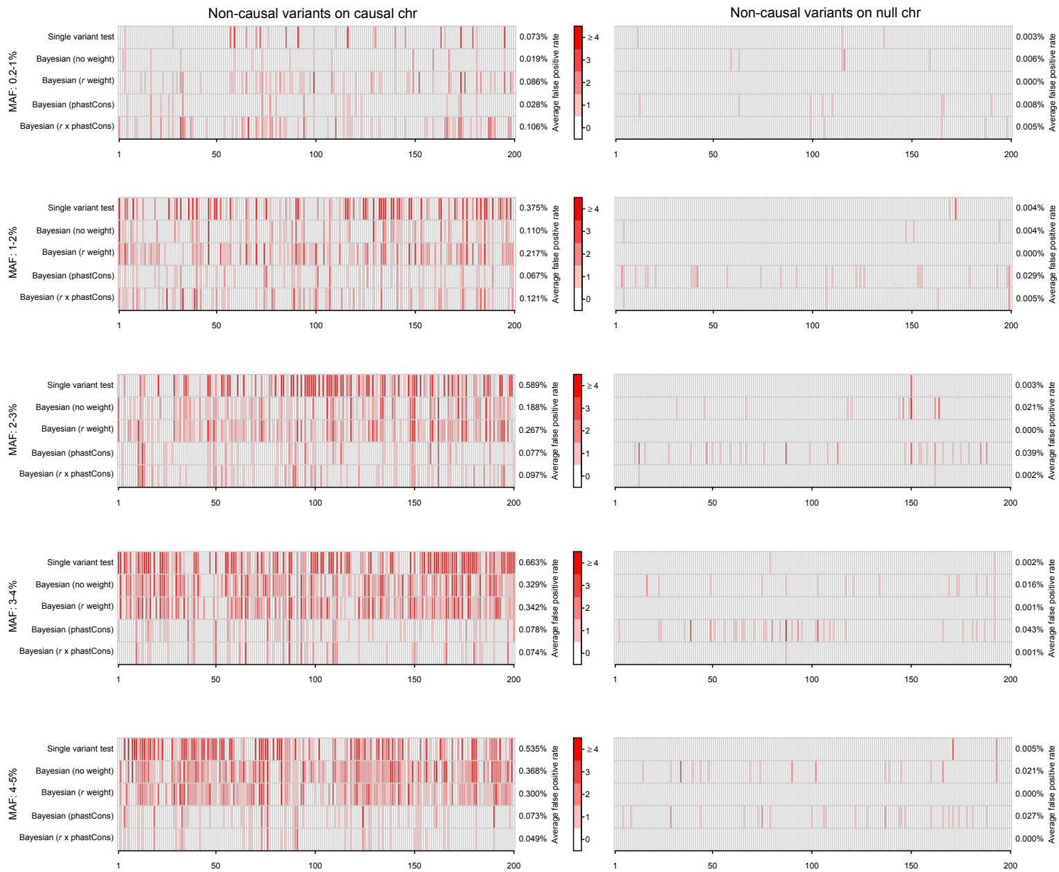
Figure S 4: Heatmap plots showing the number of non-causal variants that were falsely identified as causal in each of the 200 replicates. Numbers on the right side of each plot are false positive rates averaged across replicates for different methods.
