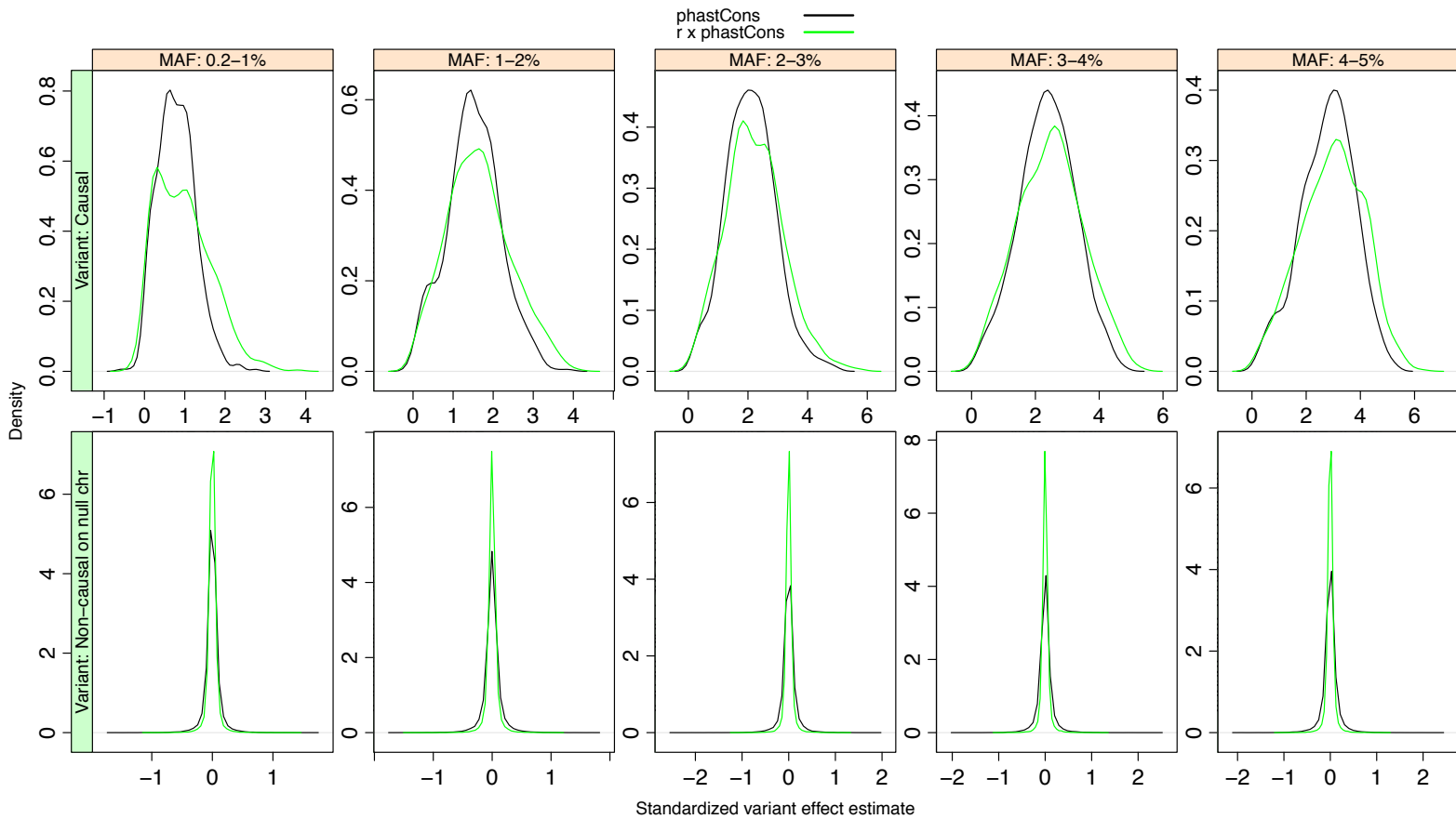
Figure S 5: Distributions of standardized variant effect estimates from Bayesian liability model with \text{phastCons} weight and with r \times \text{phastCons} weight. In each scenario (plot), effect estimates of Bayesian with \text{phastCons} weight (or r \times \text{phastCons} ) were collected from 200 replicates to form a distribution density.
