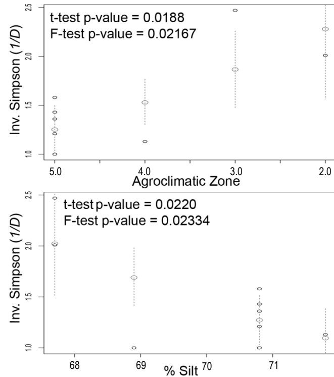
Fig. S2. The effect of soil % silt and agroclimatic zone on the diversity of phzF -containing Pseudomonas spp. communities at nine sampled IPNW sites. Diversity is represented as a function of the inverse Simpson diversity index ( 1/D ). Confidence intervals are shown as dotted lines and the plots were calculated in BiodiversityR.
