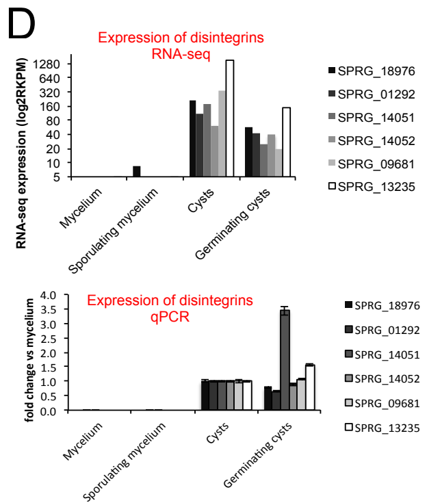
Differentially expressed genes in different life stages
