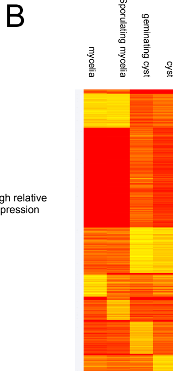
Differentially expressed genes in different life stages
