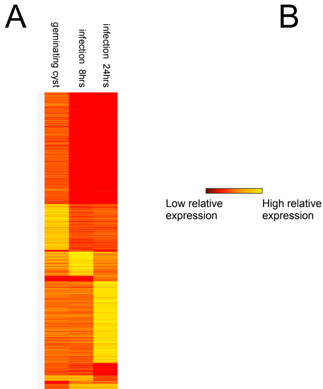
Differentially expressed genes during the infection time course
