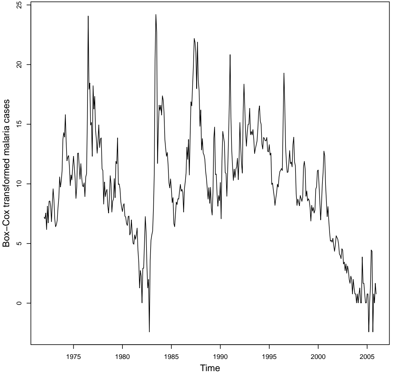
Box-Cox transformed monthly malaria case counts in Gampaha
