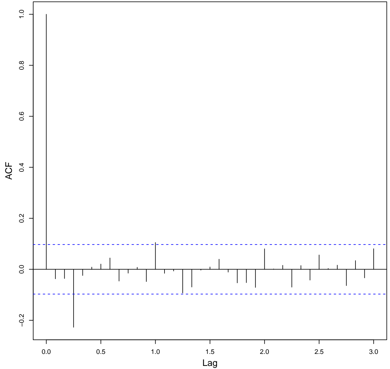
Autocorrelation function of Box-Cox transformed monthly malaria case counts in Gampaha
