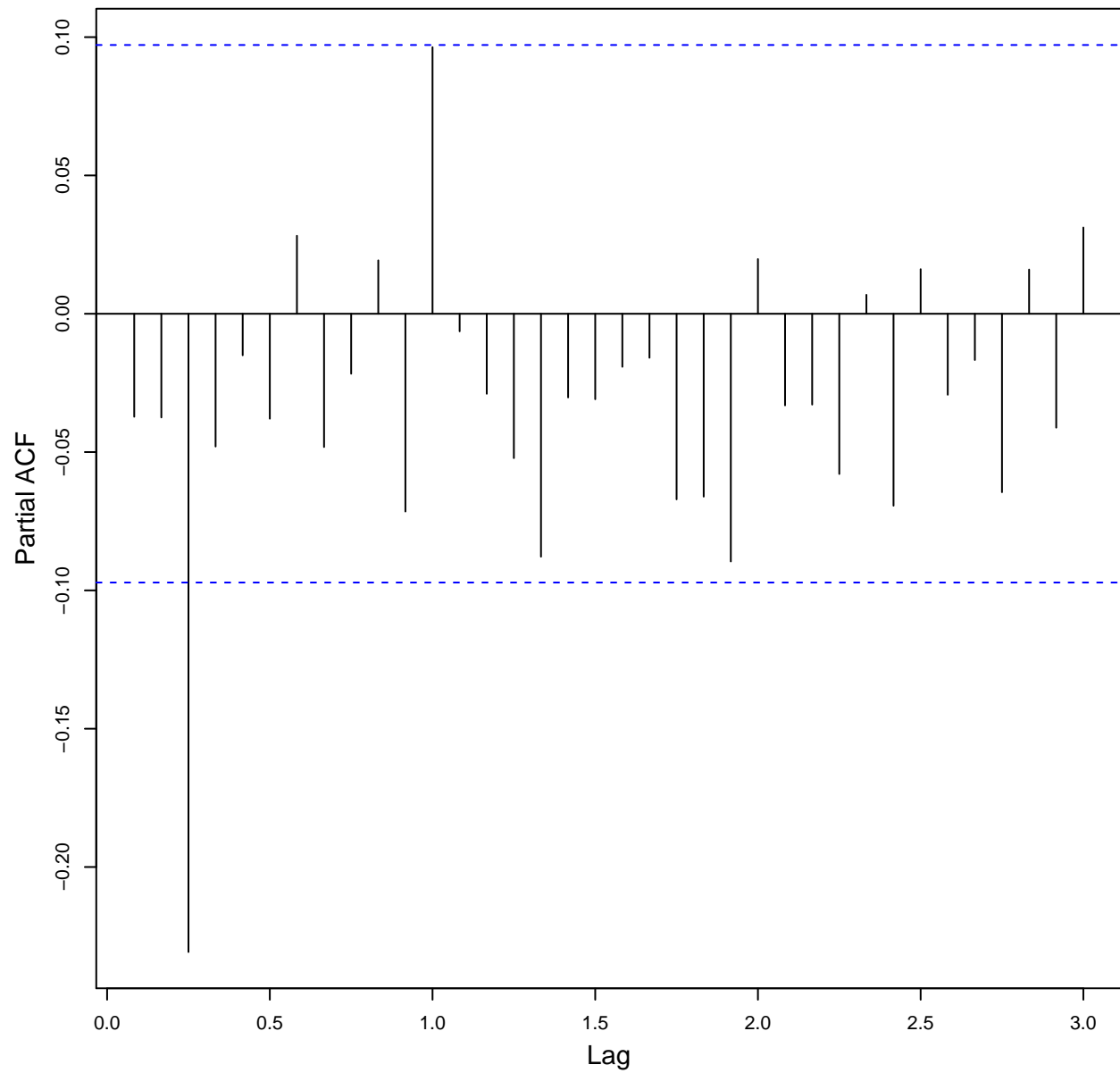
Partial autocorrelation function of Box-Cox transformed monthly malaria case counts in Gampaha
