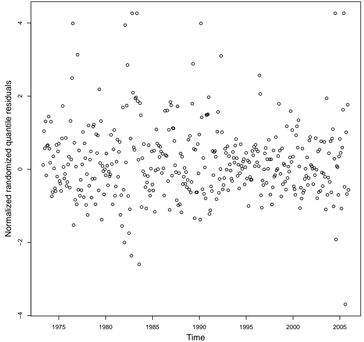
Normalized randomized quantile residuals of negative binomial GSARIMA (3', 1, 0) × (1, 0, 0) 12 model
