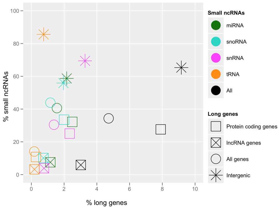
Supplementary Figure S16 Proportion of annotated elements in different genomic domains that overlap different classes of small RNAs.
