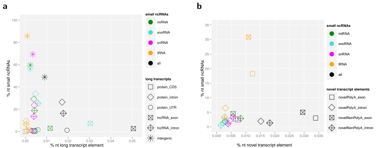
Supplementary Figure S17 Nucleotide coverage of small RNAs over long RNAs. Gencode v7 annotated small ncRNAs (miRNA, snoRNA, snRNA, tRNA) in elements (CDS, introns, UTRs, exons and intergenic regions) of a. protein coding and long noncoding transcripts and b. novel intergenic / antisense transcript models.
