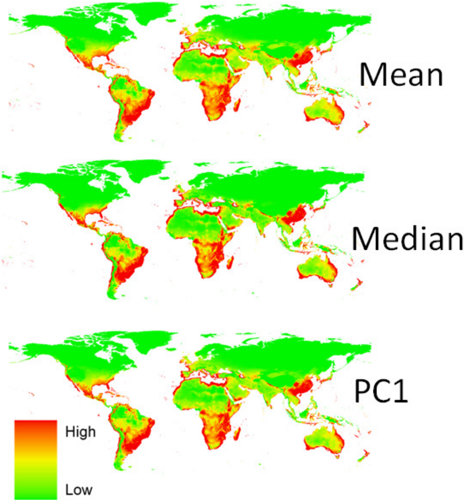
Figure S2: Results from different consensus strategies (mean, median and PCA between predictions) for current climate conditions. The three maps are fairly similar, and therefore we focused on median in the article.
