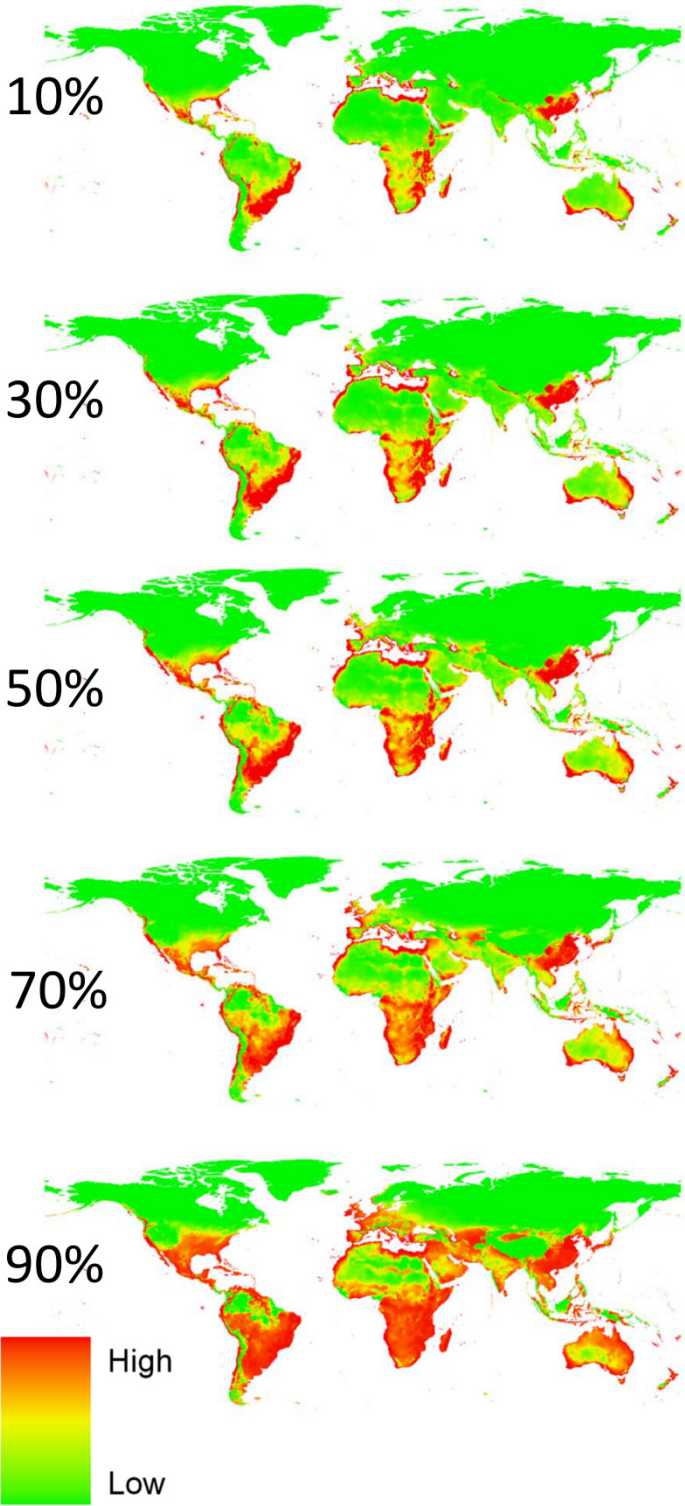
Figure S3: Model predictions using different prevalence levels under current climate conditions. Notice that the model outputs are biased in the same direction than the input prevalence, with a prevalence of 10% producing a smaller potential range than higher prevalence levels.
